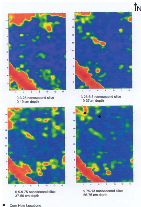
7. Amplitude time-slices of Grid 1 at the Buchtel Garden. Each slice shows the aerial extent of radar reflection amplitudes at different depths in the ground.
