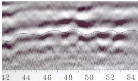
amplitude reflections.
