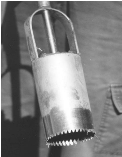
9. The hand auger used to collect complete cores of the soils at the Buchtel Chapel site.
