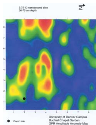
8. Amplitude slice-map from 56-75 cm in Grid 2 at the Buchtel Chapel Site.
