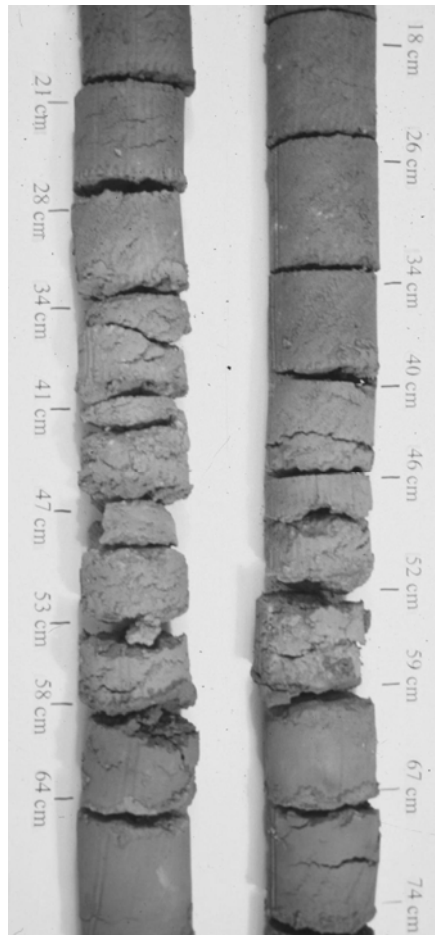
10. Cores taken both within and outside the amplitude anomaly that represents the remnant of the Buchtel Garden. The core on the left shows a \text{CaCO}_3 -rich layer at 34-58 cm depth, which is the fill that was added after the garden was removed. The core on the right recovered the same unit, but deeper and less developed. Note the sharp basal contact of the white layer in both cores at 58 centimeters depth. Below this contact is the buried A soil zone, which is all that remains of the original garden bed.
