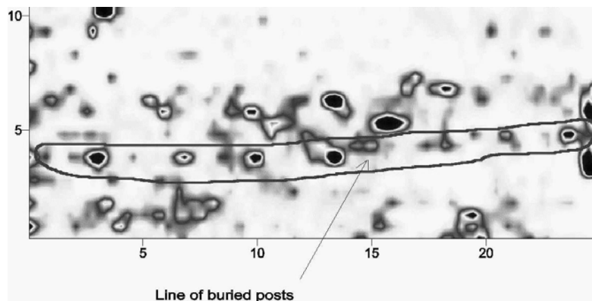
14. Buried posts from a fence at the CATS facility in Illinois. This is a slice from about 30-60 cm depth.
