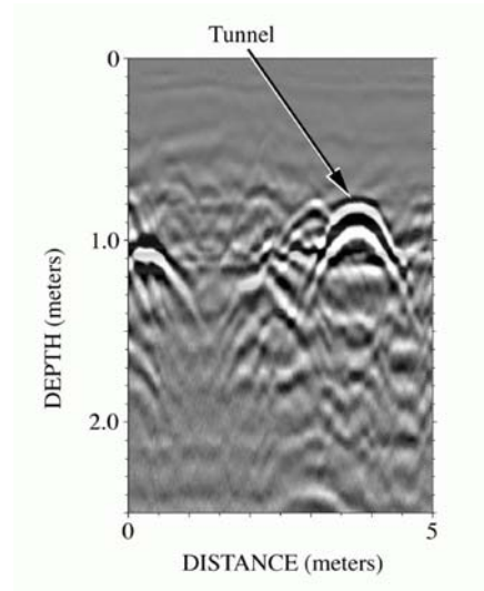
5. Example of a reflection hyperbola. In this example one created by a small tunnel
