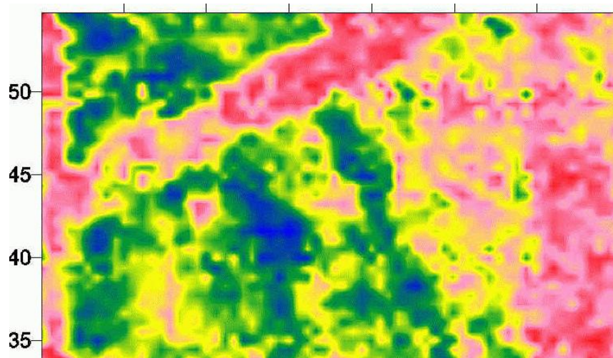
16. A buried road crosses an agricultural area at the Pio Pico historical site in Whittier, California. This map illustrates the relative amplitudes of reflected radar waves from about 40-60 cm in the ground. The compacted surface of the road is about 4 meters in width, crossing from bottom right to upper left in this image.
